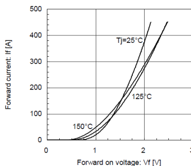
Forward Current vs. Forward Voltage (typ.) diode
